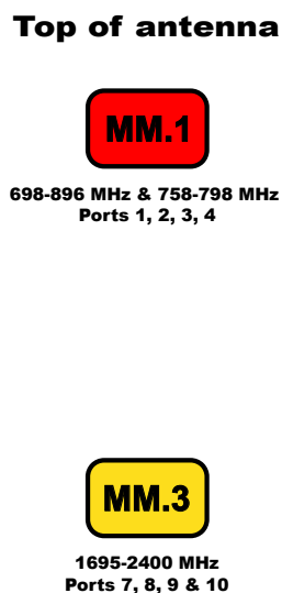
RET placement as viewed from rear of antenna
