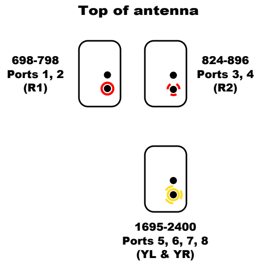
RET placement as view from rear of antenna
