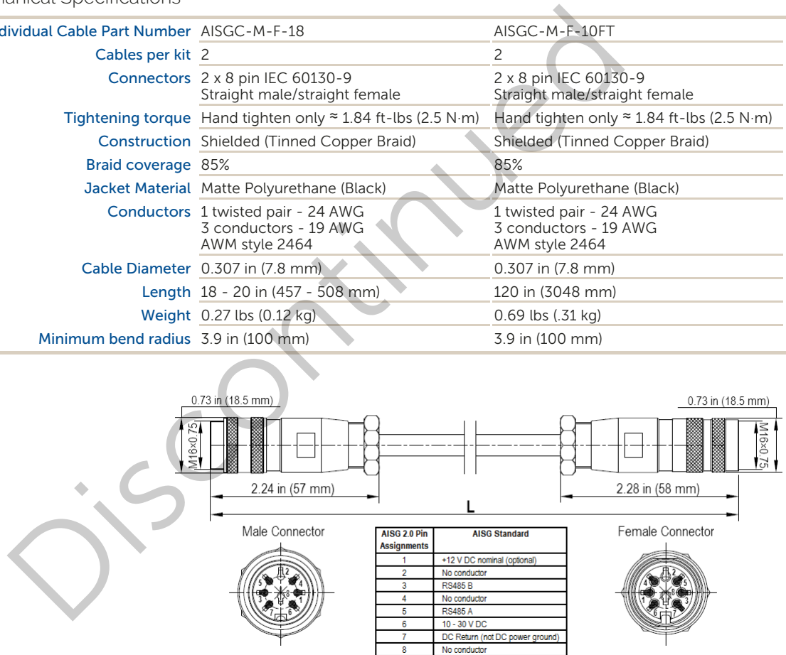
AISG-Male to AISG-Female Jumper Cable
