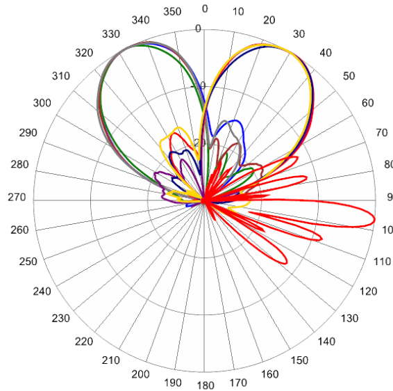
2180 MHz Azimuth with Elevation 6°
